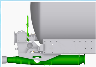
Spiral pump with stone trap and pre-equipment for front Jumbo
