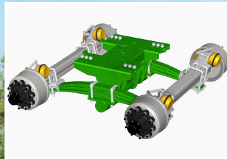
Roll-Over bogie with free-steering axle
